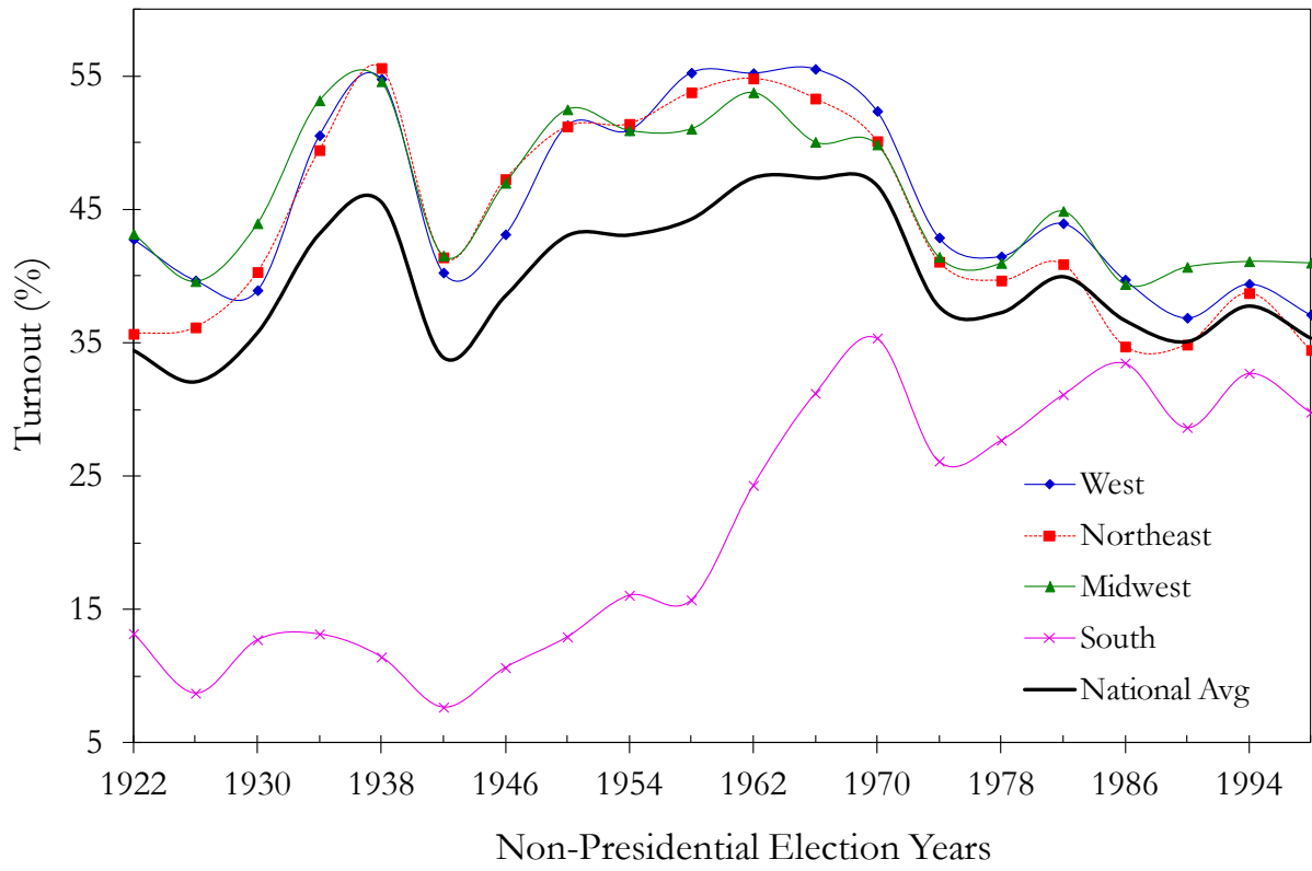
FIGURE 3.2 NONPRESIDENTIAL ELECTION YEAR VOTER TURNOUT TRENDS BY REGION, 1922-98
